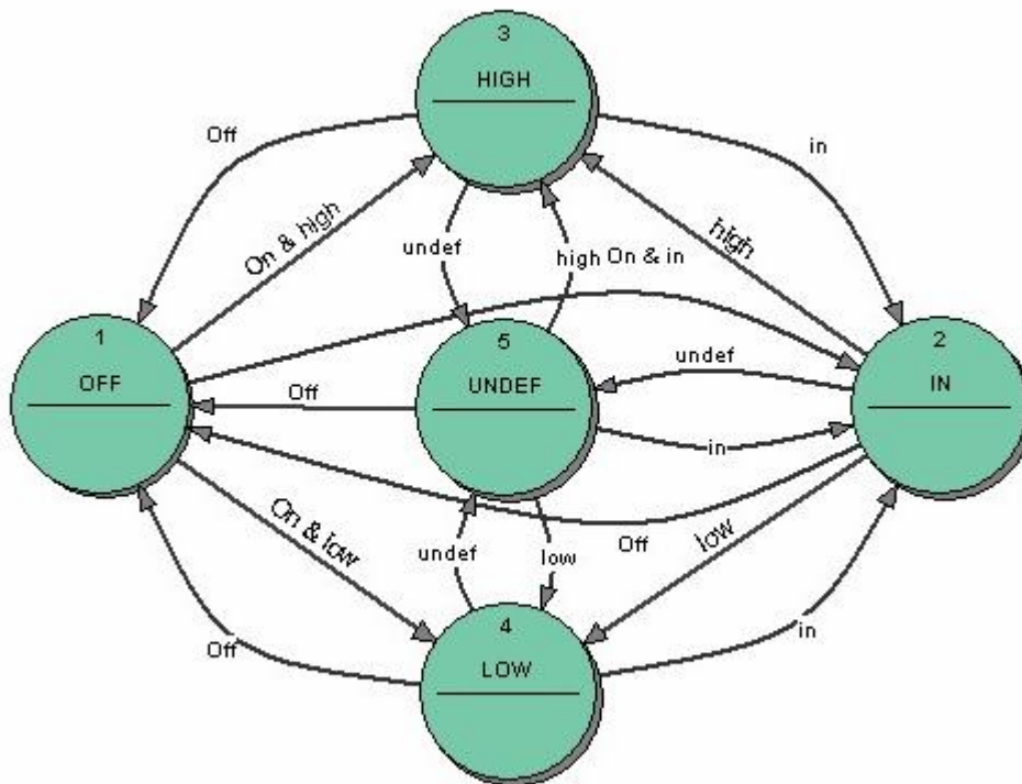
Figure 22: SWIP VFSM
