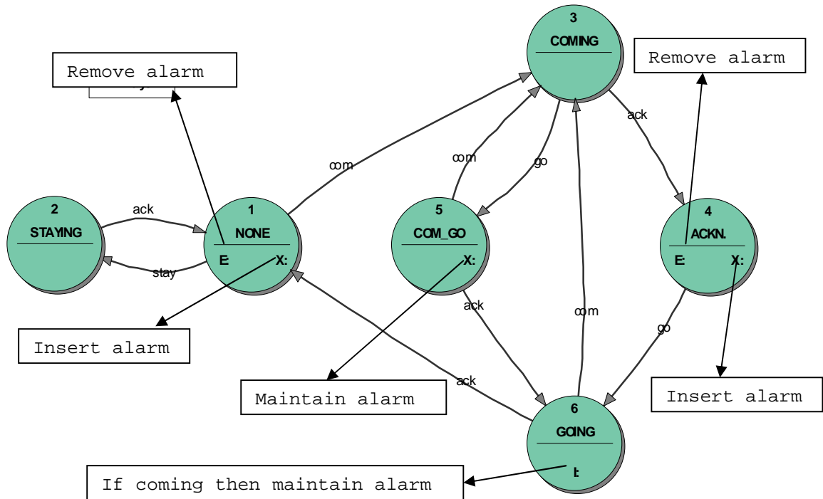
Figure 11: AL VFSM
