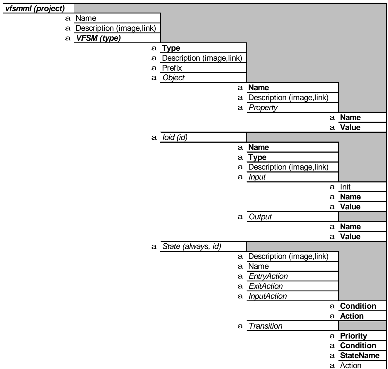
Figure 8 VFSMML tags and their hierarchy
