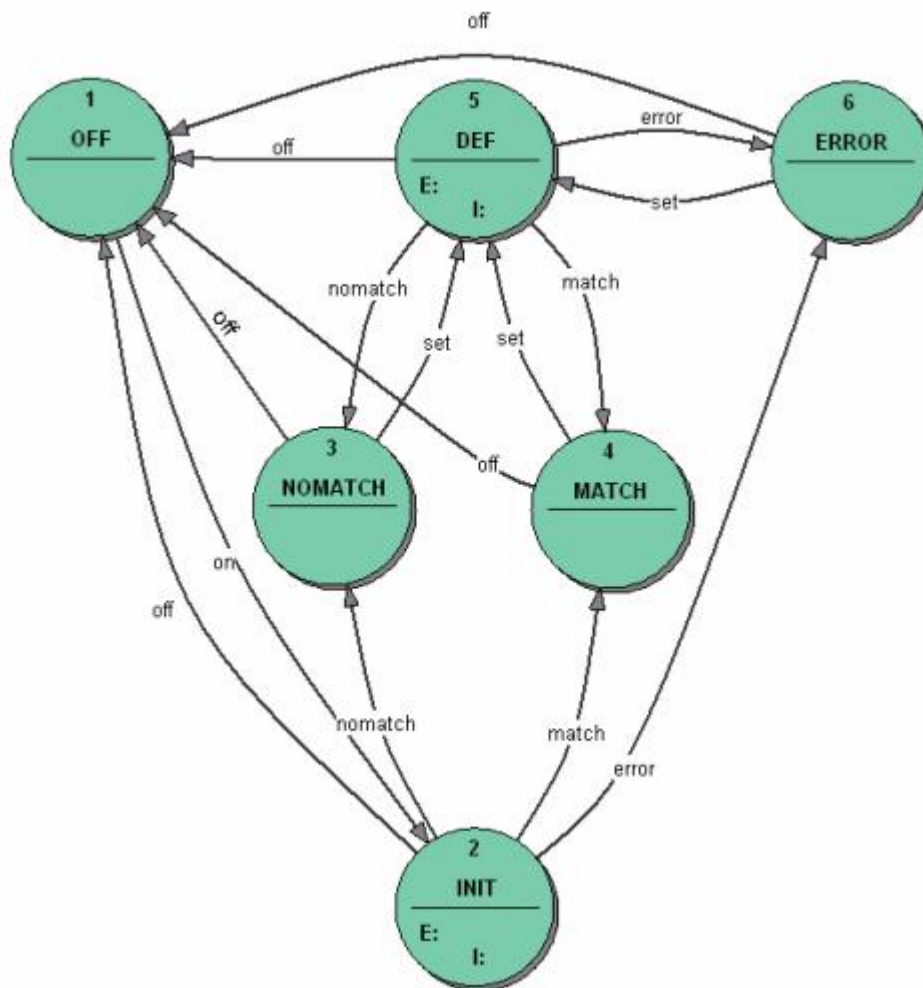
Figure 21: STR VFSM
