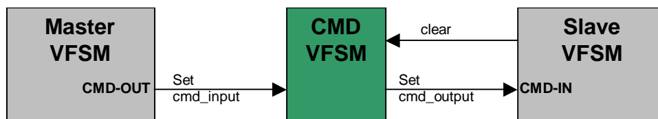
Figure 13: Usage of CMD VFSM
