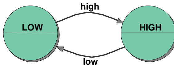
Figure 4: Digital Input (DI) object state machine
